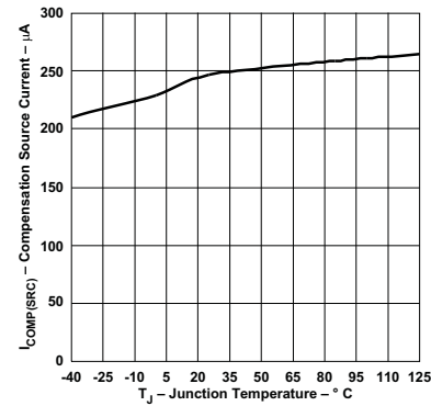
Figure 14. Compensation Source Current vs Junction Temperature
