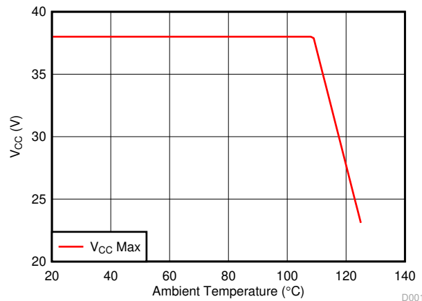
图 8-22. Power Derating Curve
