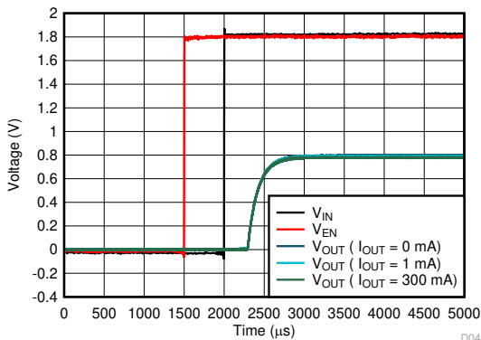
图 6-73. Start-Up Turn-On Time
