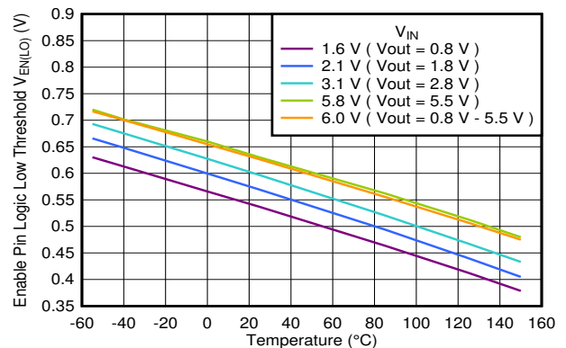
图 6-48. Enable Logic Low Threshold vs Temperature
