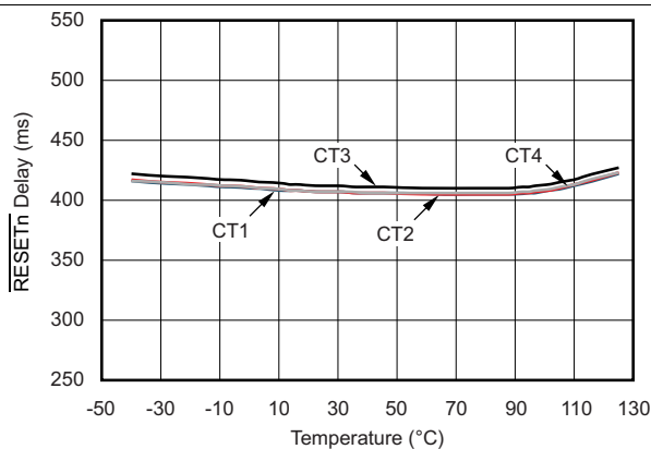
Figure 8. TPS386000-Q1 \overline{\text{RESETrn}} Timeout Period vs Temperature ( \text{CTn} = \text{Open} )
