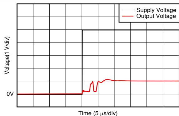
图 6-33. Start-Up Response
