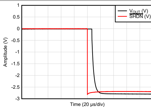
图 7-44. Amplifier Disable Response
