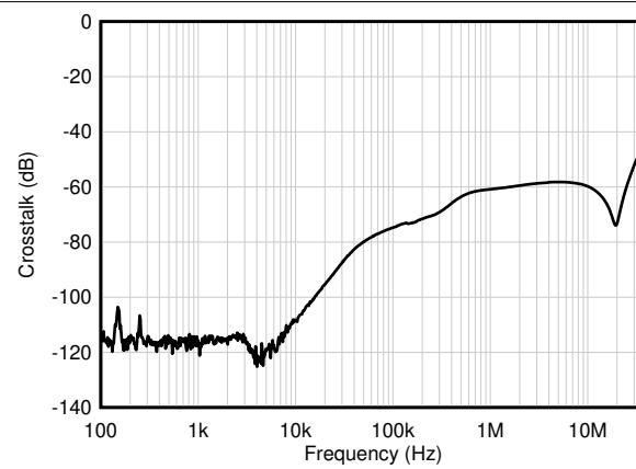
图 7-46. Channel Separation
