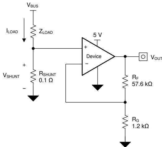
图 9-1. TLV904x in a Low-Side, Current-Sensing Application
