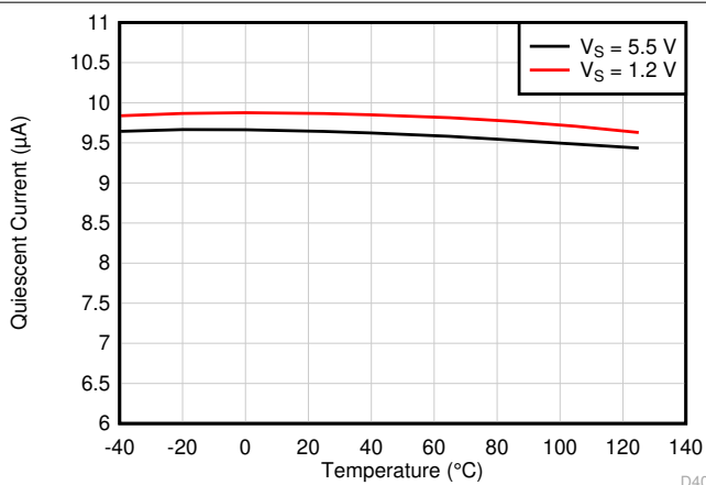
图 7-28. Quiescent Current vs Temperature
