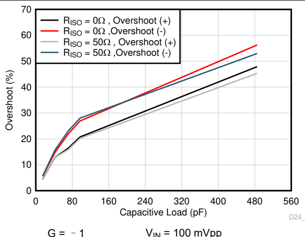
图 7-30. Small Signal Overshoot vs Capacitive Load
