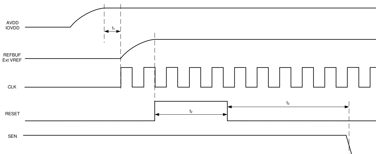
图 9-4. Initialization of Serial Registers after Power up
