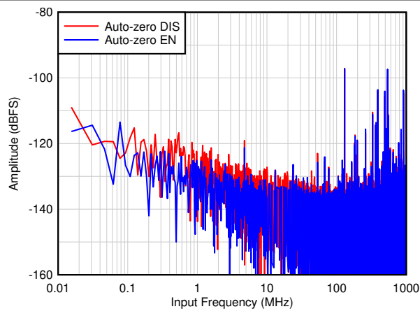
图 8-11. FFT at 65 MSPS with input frequency of 5 MHz (auto-zero feature enabled vs disabled, 4M point FFT)
