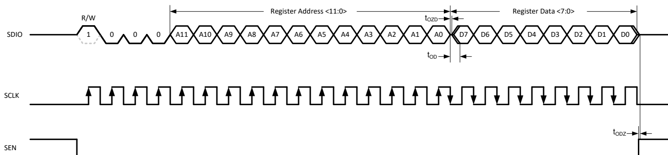
图 8-41. Serial Register Read Timing Diagram
