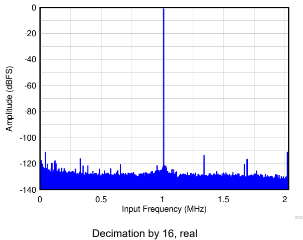
图 9-2. Single Tone FFT at F_{IN} = 1 MHz
