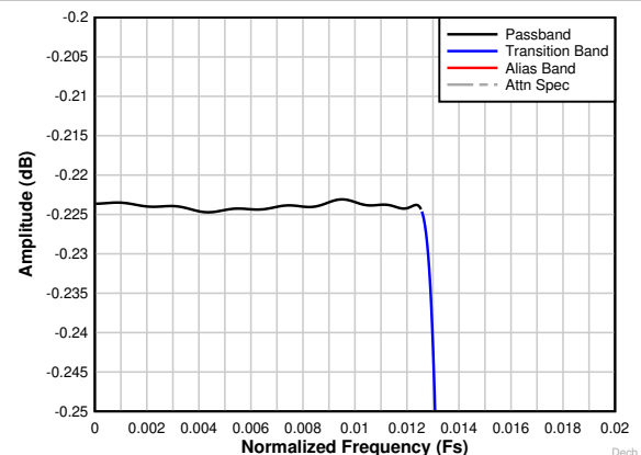
图 8-32. Decimation by 32 complex passband ripple response
