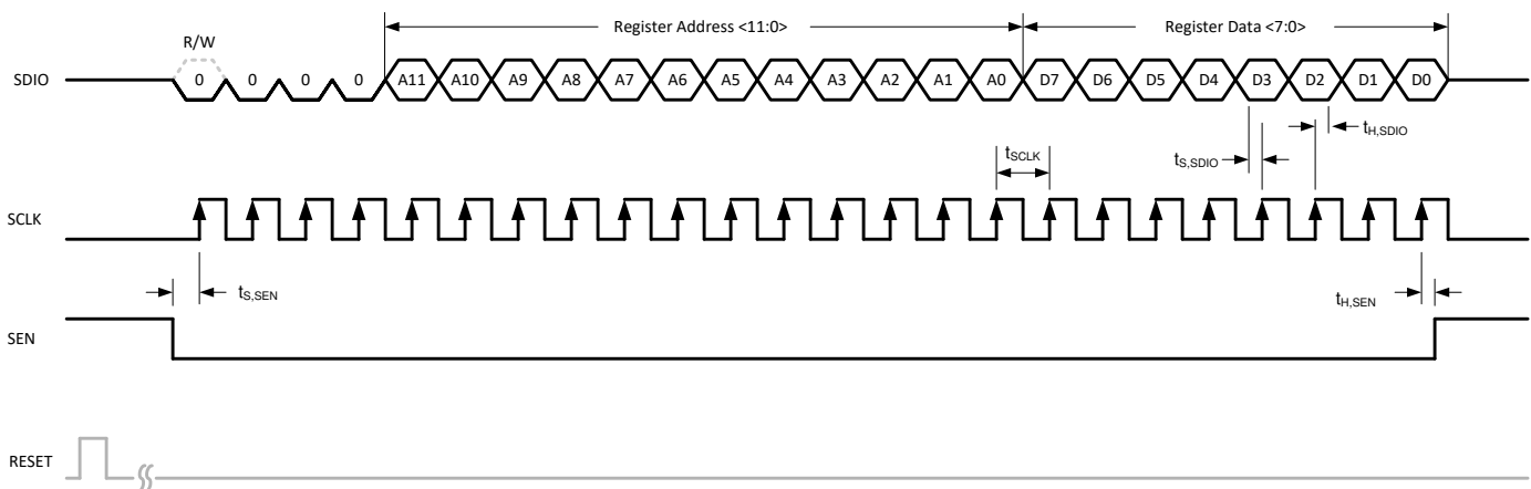
图 8-40. Serial Register Write Timing Diagram
