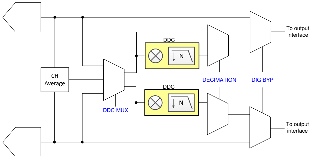
图 8-58. Register control for digital features
