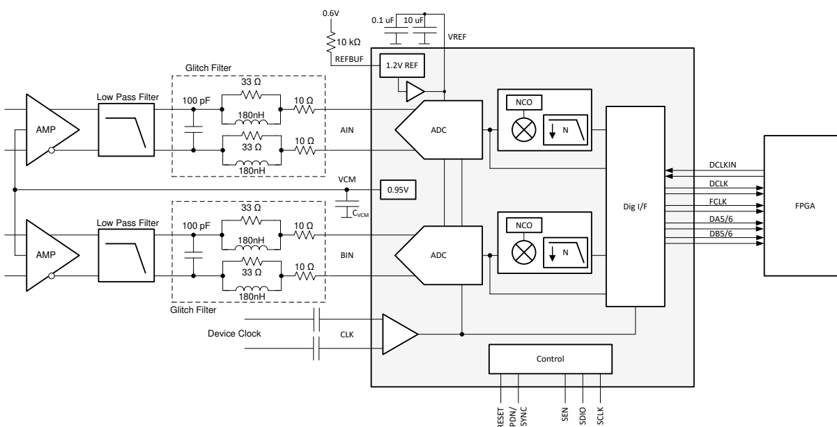
图 9-1. Typical configuration for a spectrum analyzer with DC support
