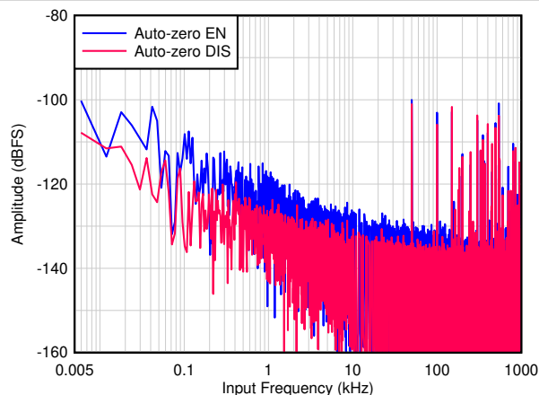
图 8-9. FFT at 25 MSPS with input frequency of 5 MHz (auto-zero feature enable vs disable, 4M point FFT)
