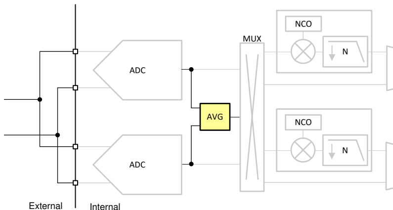
图 8-39. Digital Channel Averaging Diagram
