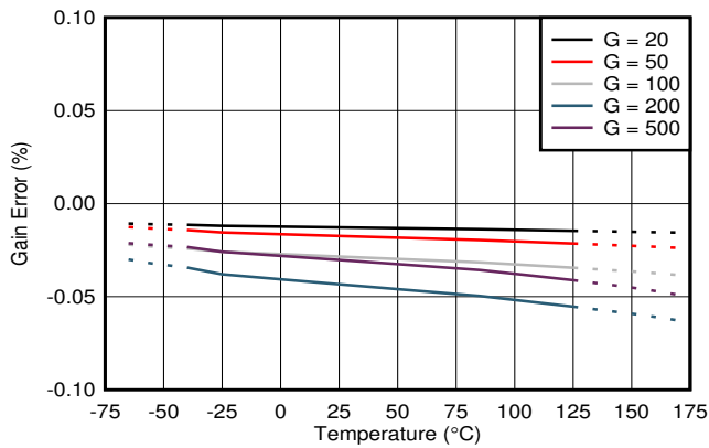
图 6-11. Gain Error vs. Temperature
