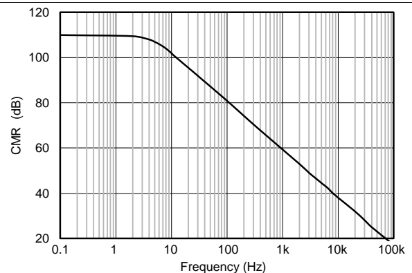
Figure 18. Common-Mode Rejection vs Frequency V_S = 5\text{ V} , V_{REF} = 2.5\text{ V} , I_{SENSE} = 0\text{ A} , V_{CM} = 1\text{-V sine wave}
