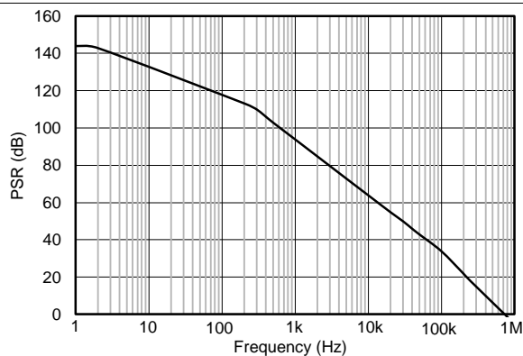
Figure 17. Power-Supply Rejection vs Frequency V_{CM} = 12\text{ V} , V_{REF} = 2.5\text{ V} , I_{SENSE} = 0\text{ A} , V_S = 5\text{ V} + 250\text{-mV sine disturbance}
