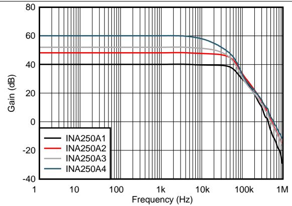
Figure 16. Amplifier Gain vs Frequency V_{CM} = 12\text{ V} , I_{SENSE} = 500\text{ mA}_{PP}
