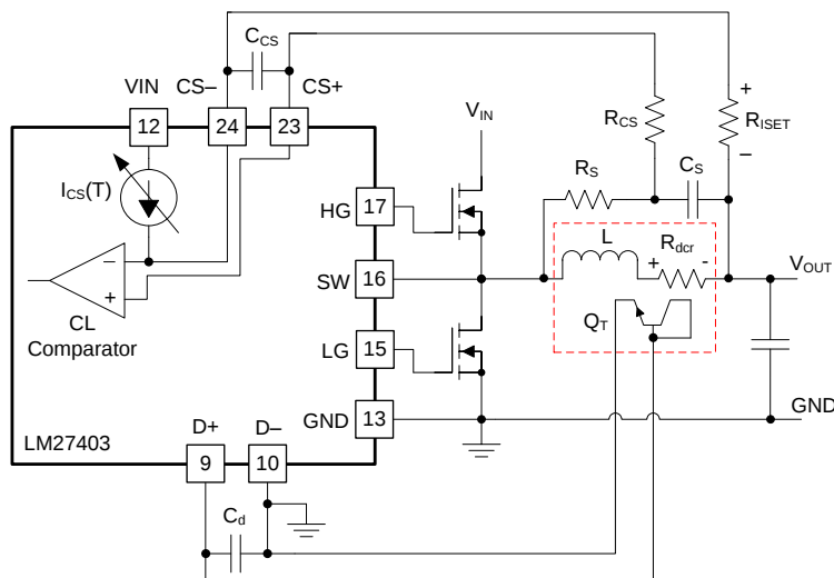
图 32. Current-Limit Setpoint Defined by Current Source I_{CS} and Resistor R_{SET}
