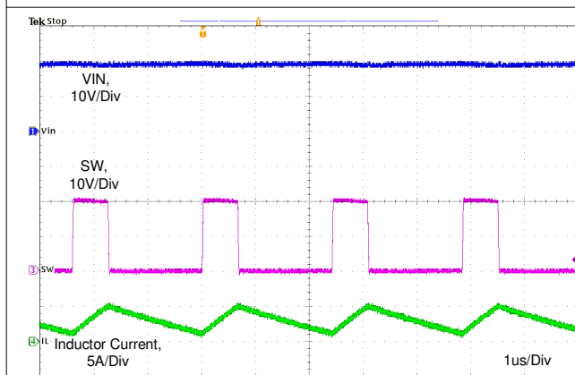
A. V_{IN} = 20 \text{ V} L = 2.2 \text{ }\mu\text{H} I_{LOAD} = 3 \text{ A}
