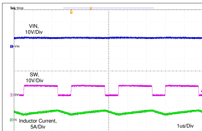
A. V_{IN} = 7.5 \text{ V} L = 2.2 \text{ }\mu\text{H} I_{LOAD} = 3 \text{ A}
