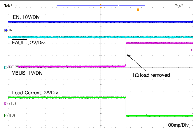
Figure 11-21. Short Circuit Recovery Without External FET
