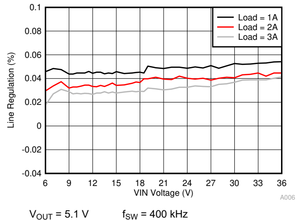
Figure 11-7. Line Regulation
