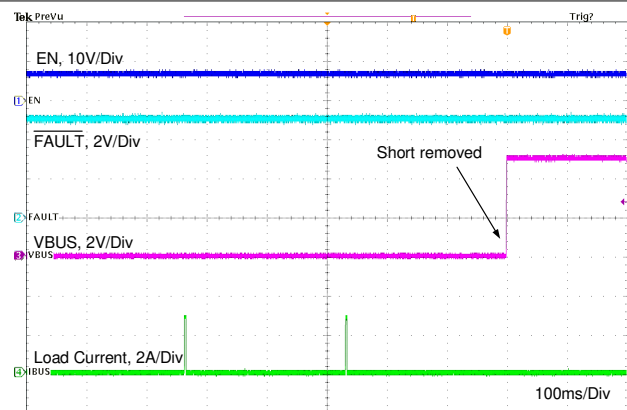
Figure 11-23. 1-Ω Load Recovery Without External FET
