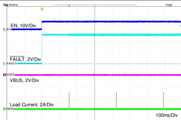
Figure 11-22. Enable Into 1-Ω Load Without External FET
