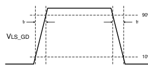
Figure 9-2. NFET Gate Drive Rise and Fall Time
