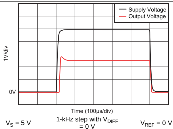
图 21. Start-Up Response
