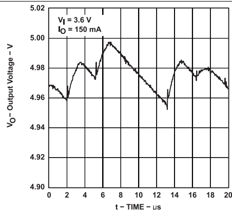
Figure 25. Output Voltage Ripple vs Time
