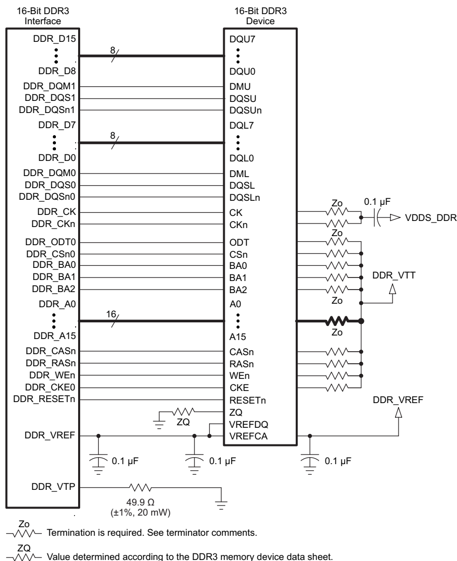
Figure 5-49. 16-Bit DDR3 Interface Using One 16-Bit DDR3 Device With V_{\text{TT}} Termination
