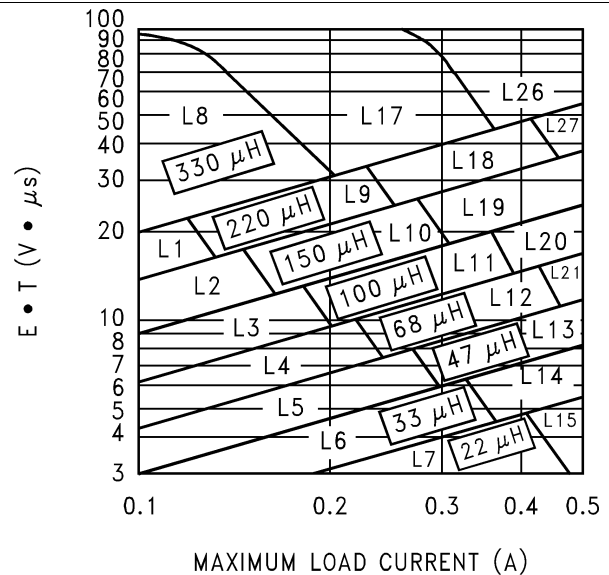
Figure 41. LM2597xx Adjustable Voltage Version
