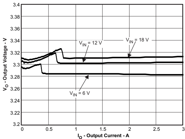
Figure 4. V_O=3.3\text{V} Output Voltage vs Output Current
