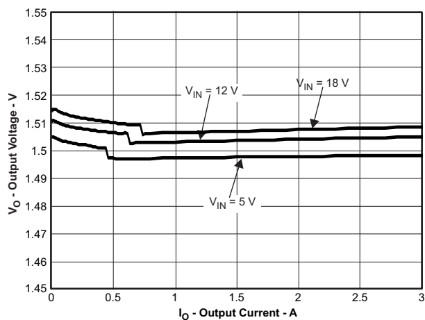
Figure 5. V_O=1.5\text{V} Output Voltage vs Output Current
