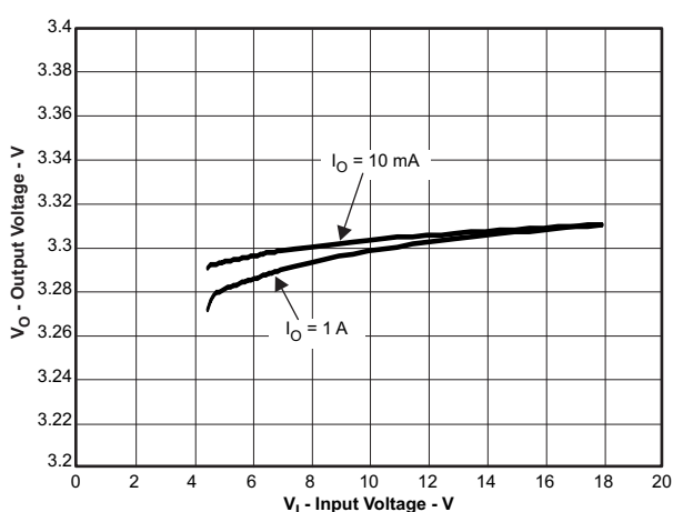
Figure 6. V_O=3.3\text{V} Output Voltage vs Input Voltage
