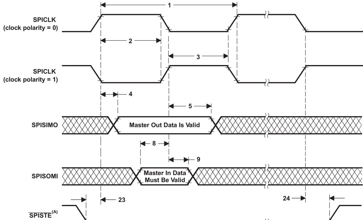
图 5-71. SPI Master Mode External Timing (Clock Phase = 0)
