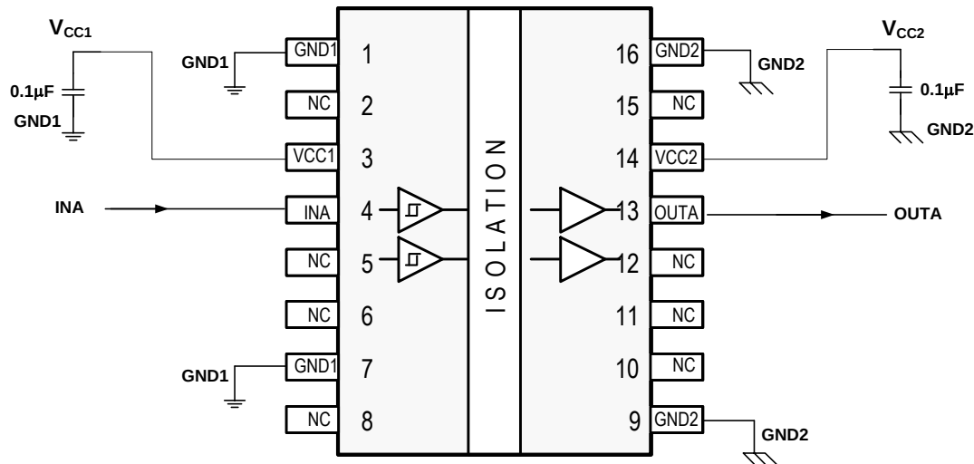
Figure 16. Typical ISO7810DW Circuit Hook-up
