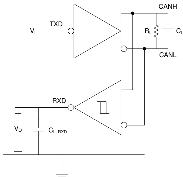
图 8-8. Loop Delay Symmetry Test Circuit and Measurement
