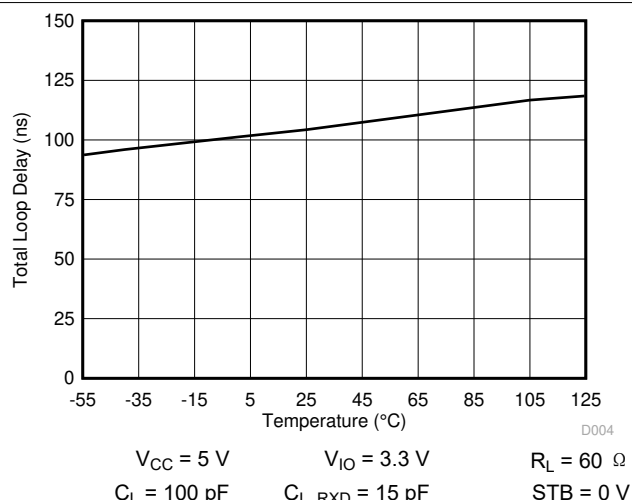
图 7-4. Total Loop Delay over Temperature
