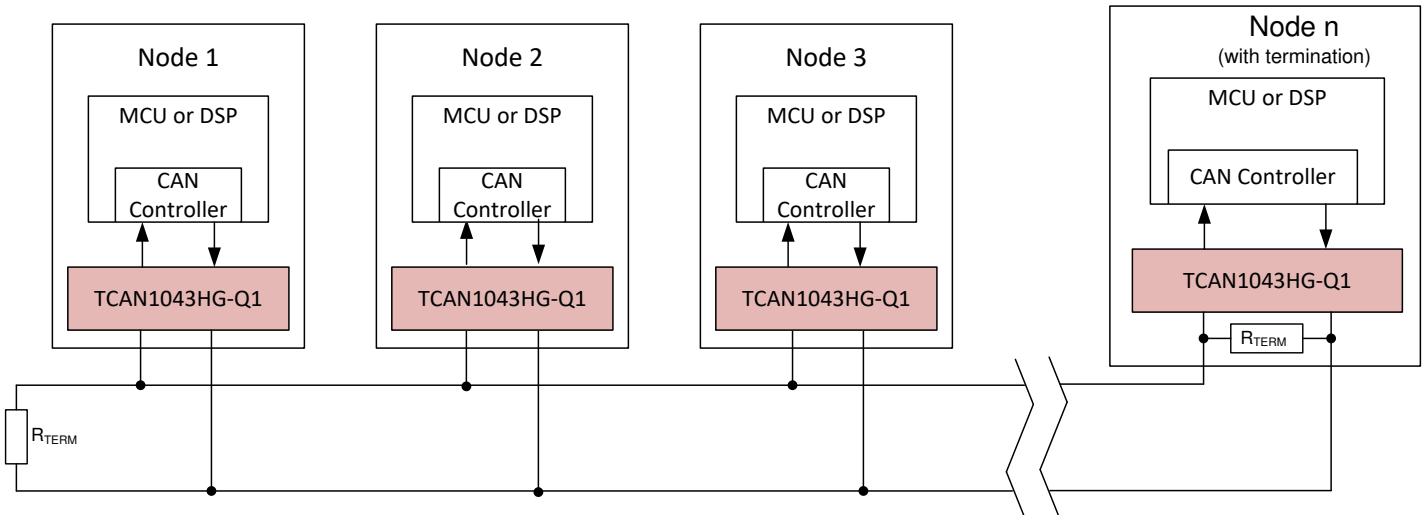
图 10-3. Typical CAN Bus Application
