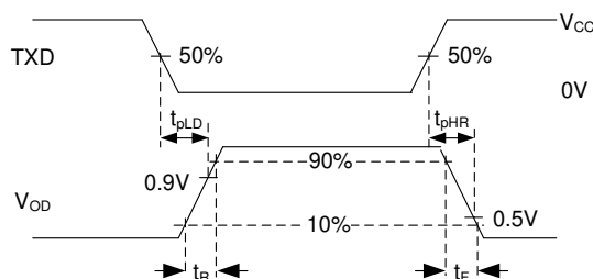
图 8-2. Driver Test Circuit and Measurement
