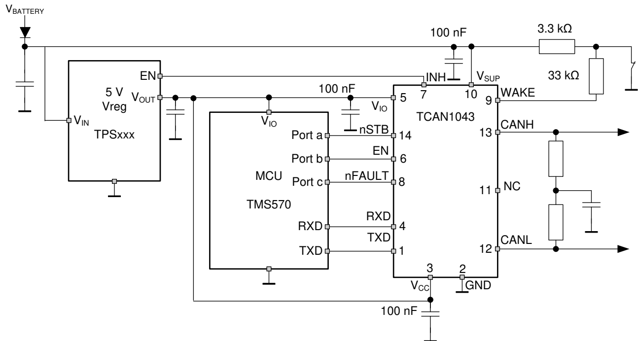
图 10-1. Typical CAN Bus Application Using TCAN1043xx-Q1 with 5 V \mu C
