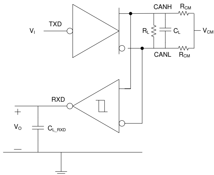
图 8-6. t_{\text{PROP(LOOP)}} Test Circuit and Measurement
