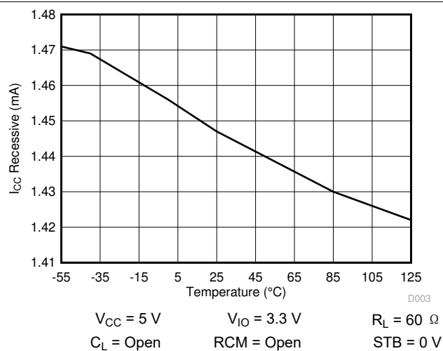
图 7-3. I_{CC} Recessive over Temperature
