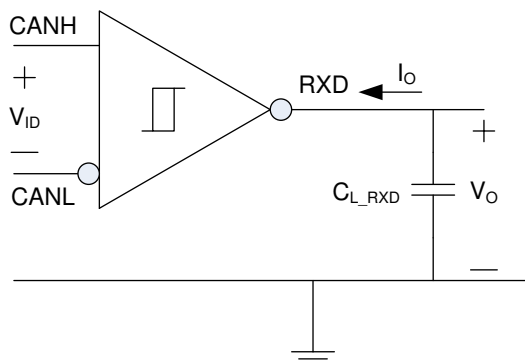
图 8-3. Receiver Test Circuit and Measurement
