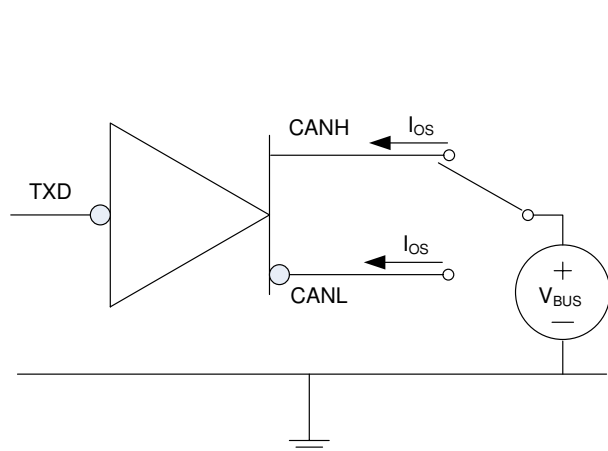
图 8-9. TXD Dominant Timeout Test Circuit and Measurement
