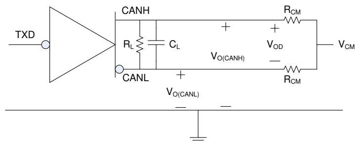
图 8-2. Driver Test Circuit and Measurement
