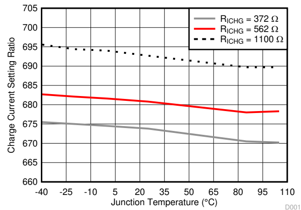
Figure 8-7. Charge Current Setting Ratio vs. Junction Temperature
