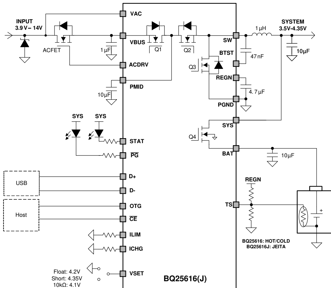
Figure 10-22. BQ25616/616J Application Diagram with External OVP
