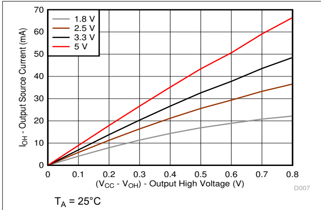
图 6-7. Source Current ( I_{OH} ) vs Output High Voltage ( V_{OH} ) for P-Ports at Four Supply Voltages
