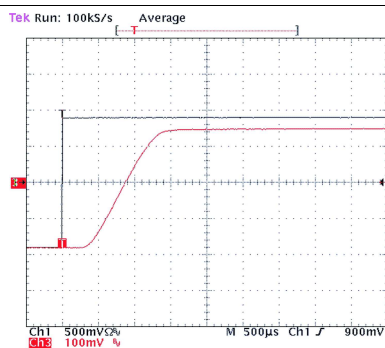
Figure 36. Turn-On Response
