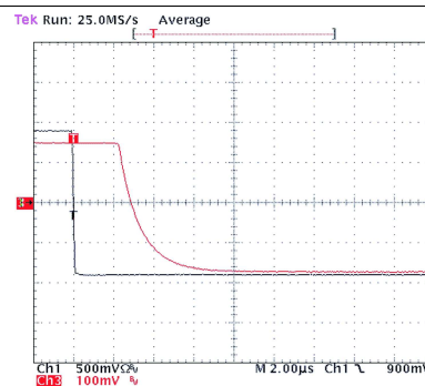
Figure 37. Turn-Off Response
