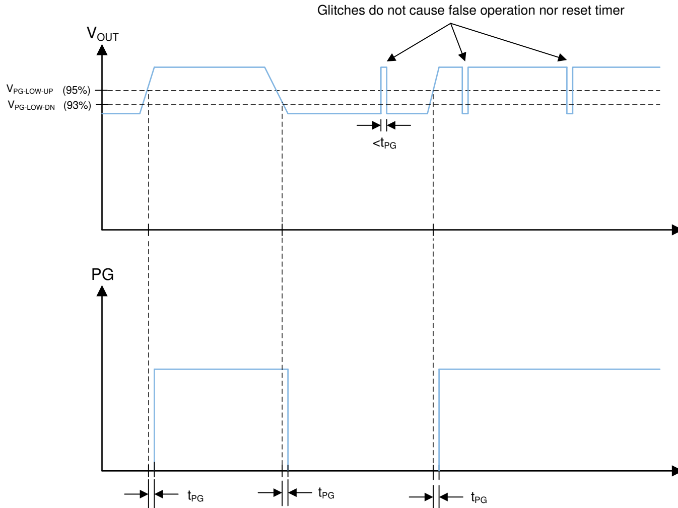
图 9. Power-Good-Timing Behavior
