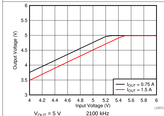
图 48. Overall Dropout Characteristic
