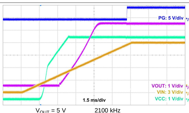
图 51. Start-Up Waveform
