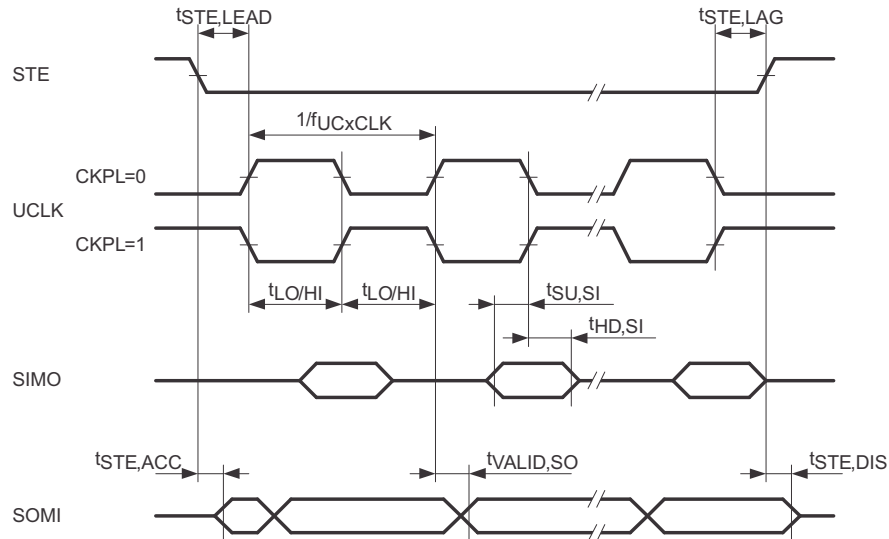
Figure 5-20. SPI Slave Mode, CKPH = 0
