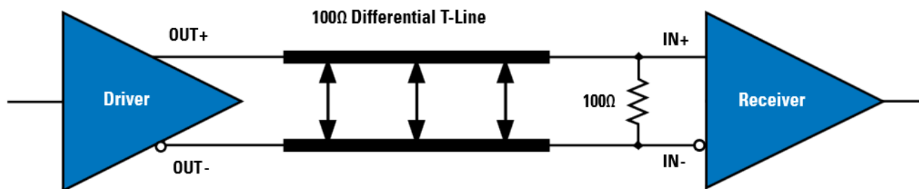
Figure 18. Point-to-Point Topology
