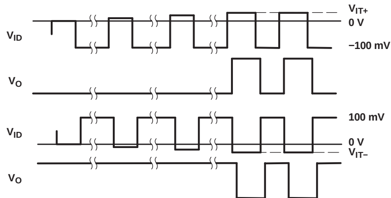
Figure 12. V_{IT+} and V_{IT-} Input Voltage Threshold Test Circuit and Definitions
