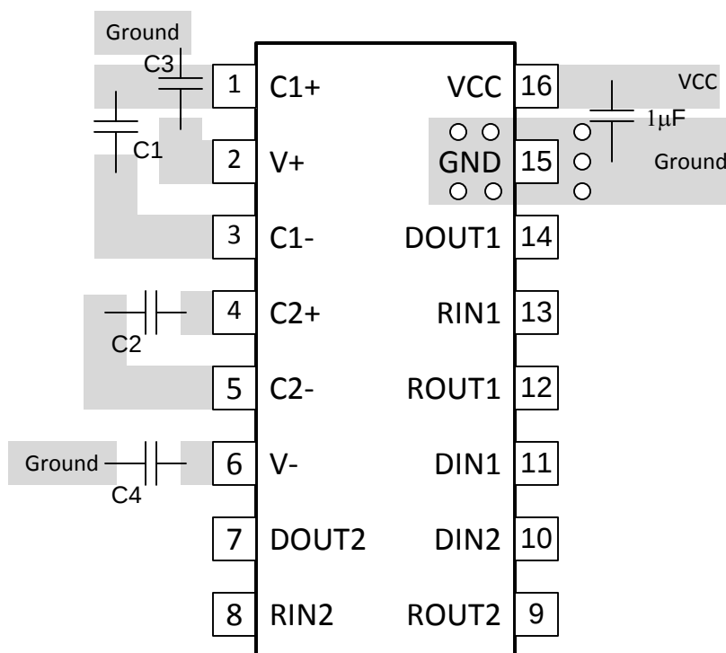
Figure 11. TRS202E Layout
