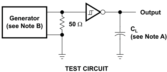
Figure 8. Receiver Propagation Delay Times
