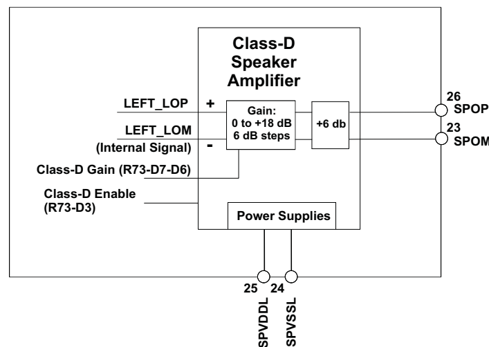
Figure 39. Differential Class-D Speaker Circuit
