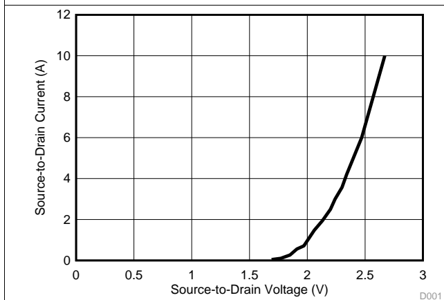
Figure 3. Source-to-Drain Current vs Source-to-Drain Voltage
