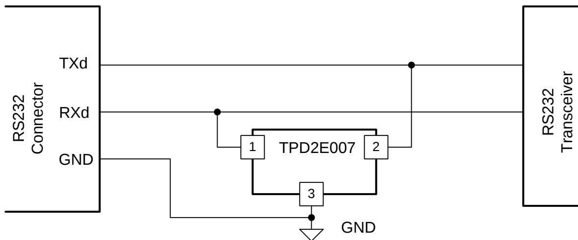
Figure 6. Example Schematic
