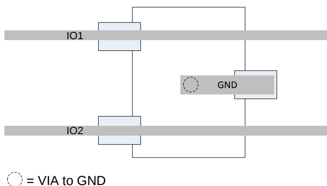
Figure 8. Layout Recommendation
