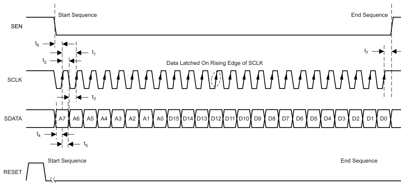
Figure 57. SPI Timing
