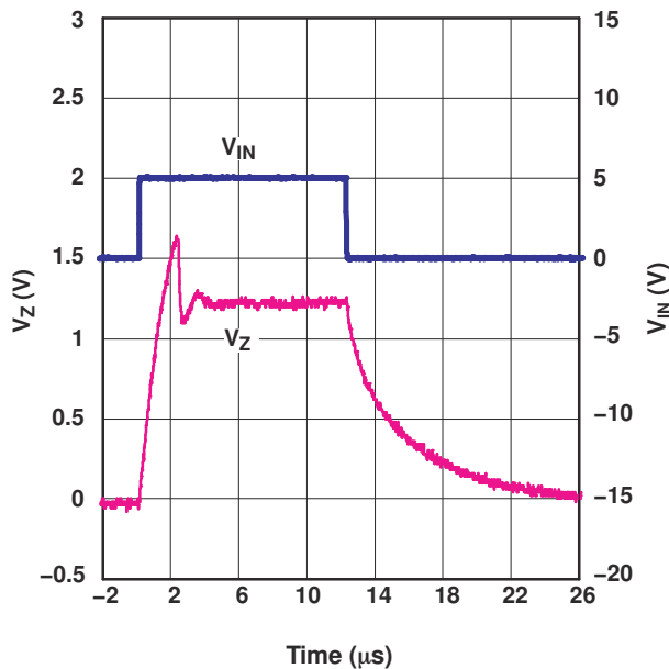
图 13-3. Start-Up Characteristics
