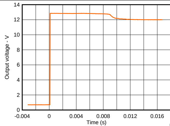
Figure 14. Output Response With De-Activation of Coil (Turn Off)
