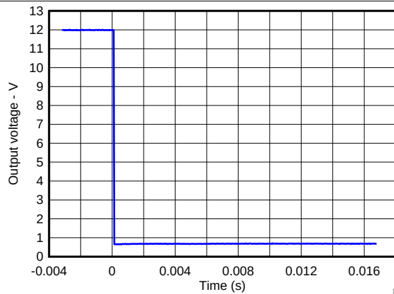
Figure 13. Output Response With Activation of Coil (Turn On)
