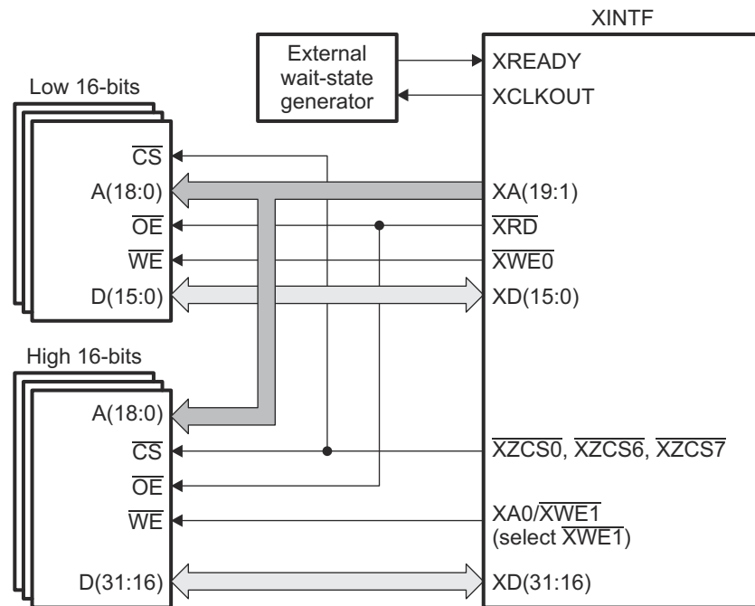
图 8-22. Typical 32-Bit Data Bus XINTF Connections
