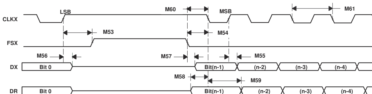
图 7-26. McBSP Timing as SPI Master or Slave: CLKSTP = 11b, CLKXP = 1
