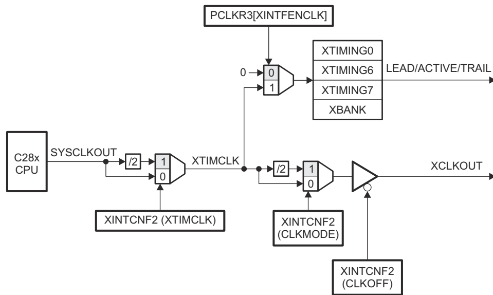
图 7-28. Relationship Between SYSCCLKOUT and XTIMCLK
