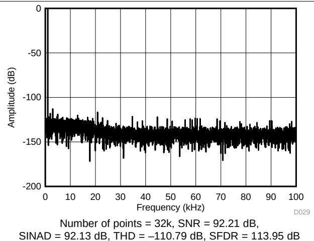
Figure 33. Typical FFT Plot ( \pm 5\text{ V} )
