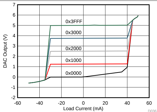
Figure 34. Source and Sink Capability with Gain = 1/2
