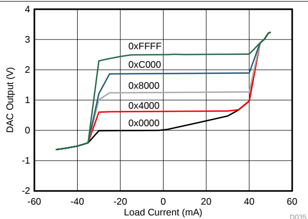
Figure 33. Headroom/Footroom vs Load Current
