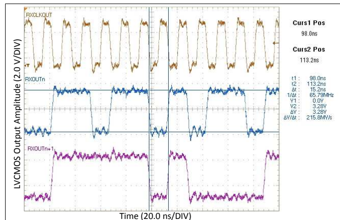
Figure 12. Parallel PRBS-7 on LVCMOS Outputs at 66 MHz
