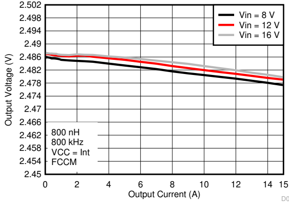
图 8-8. Output Voltage vs Output Current
