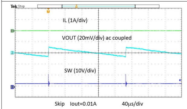
图 8-30. Output Voltage Ripple, Skip
