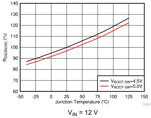
图 6-13. R_{DS(on)(HS)} vs Junction Temperature
