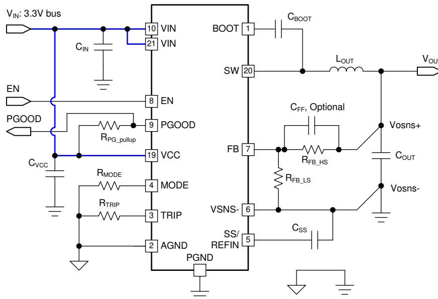
图 7-5. Single VIN Configuration With 3.3-V Bus
