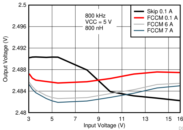
图 8-12. Output Voltage vs Input Voltage VCC = 5.0V External Bias
