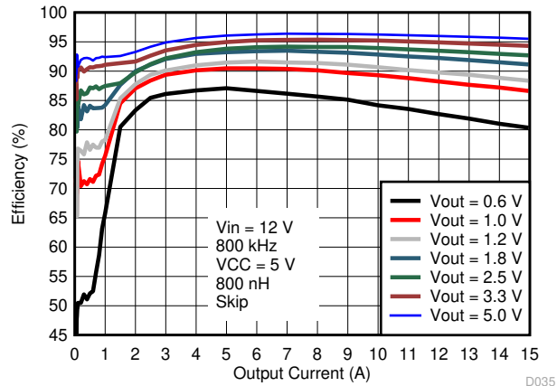
图 8-3. Efficiency vs Output Current, VCC = 5.0V External VCC Bias
