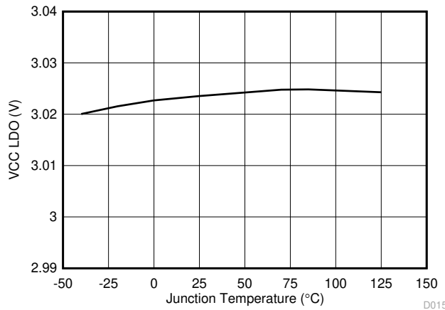
图 6-9. VCC LDO vs Junction Temperature
