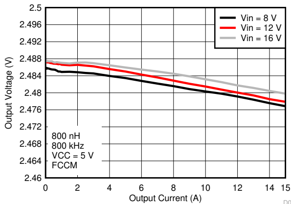
图 8-10. Output Voltage vs Output Current, VCC = 5.0V External Bias
