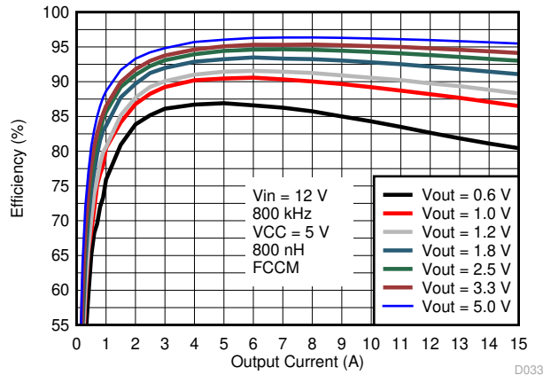
图 8-2. Efficiency vs Output Current, VCC = 5.0V External VCC Bias
