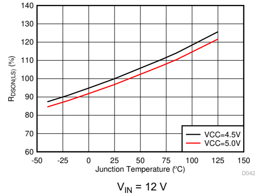
图 6-14. R_{DS(on)(LS)} vs Junction Temperature
