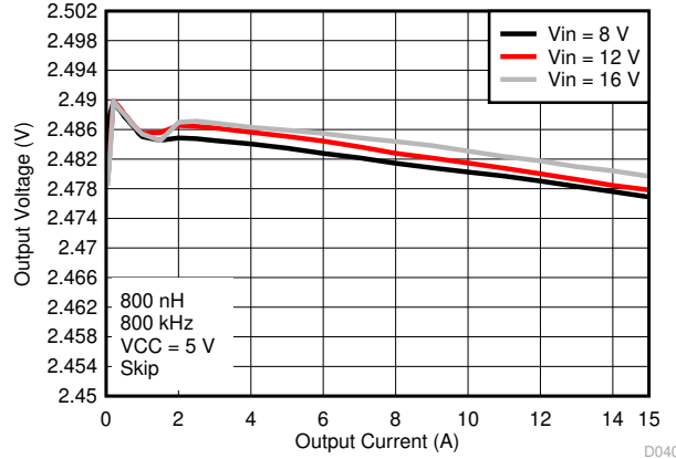
图 8-9. Output Voltage vs Output Current, VCC = 5.0V External Bias
