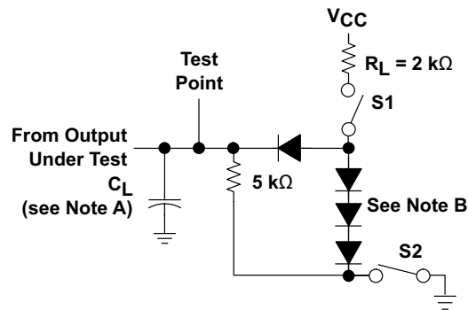
Figure 11. Test Circuit
