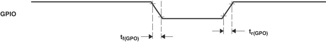
图 8-56. General-Purpose Output Timing
