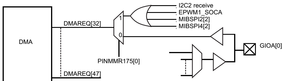
图 6-19. Using a GPIO terminal as a DMA Request Input
