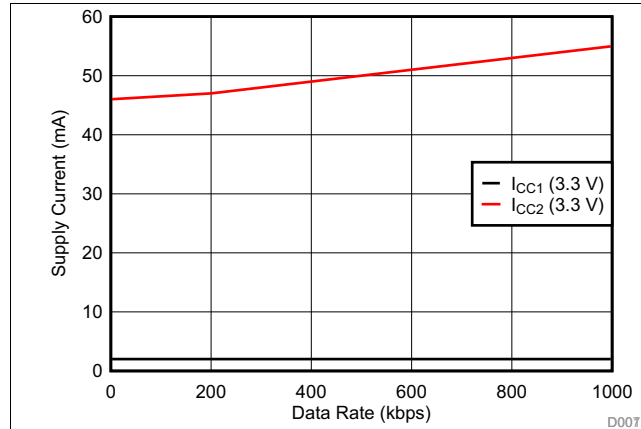
Figure 1. ISOx5 Supply Current vs Data Rate With Load
