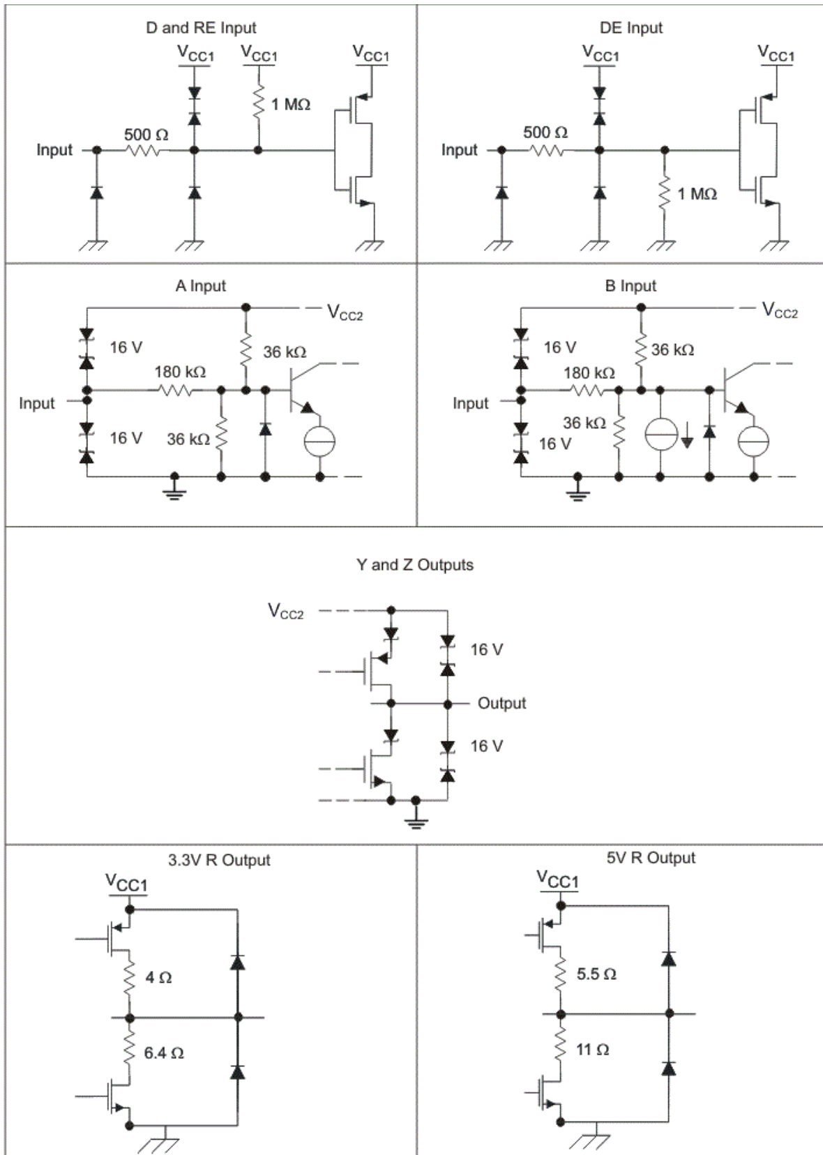
Figure 17. Device I/O Schematics
