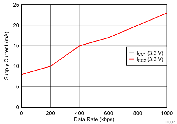
Figure 2. ISOx5 Supply Current vs Data Rate With No Load
