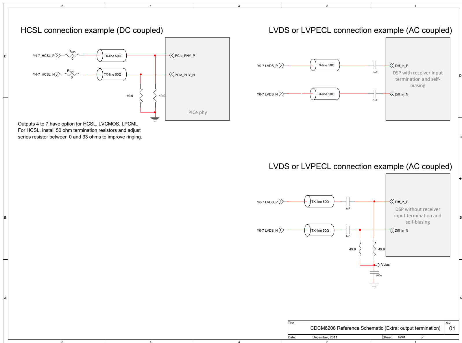
Figure 64. Schematic Page 4
