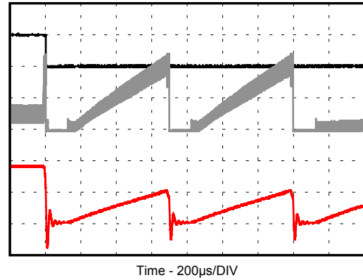
图 9-34. HICCUP Short Circuit Protection
