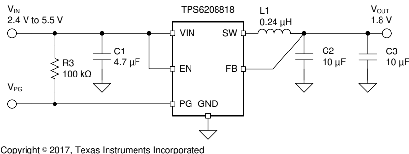
图 9-2. Typical Application of Fixed Output
