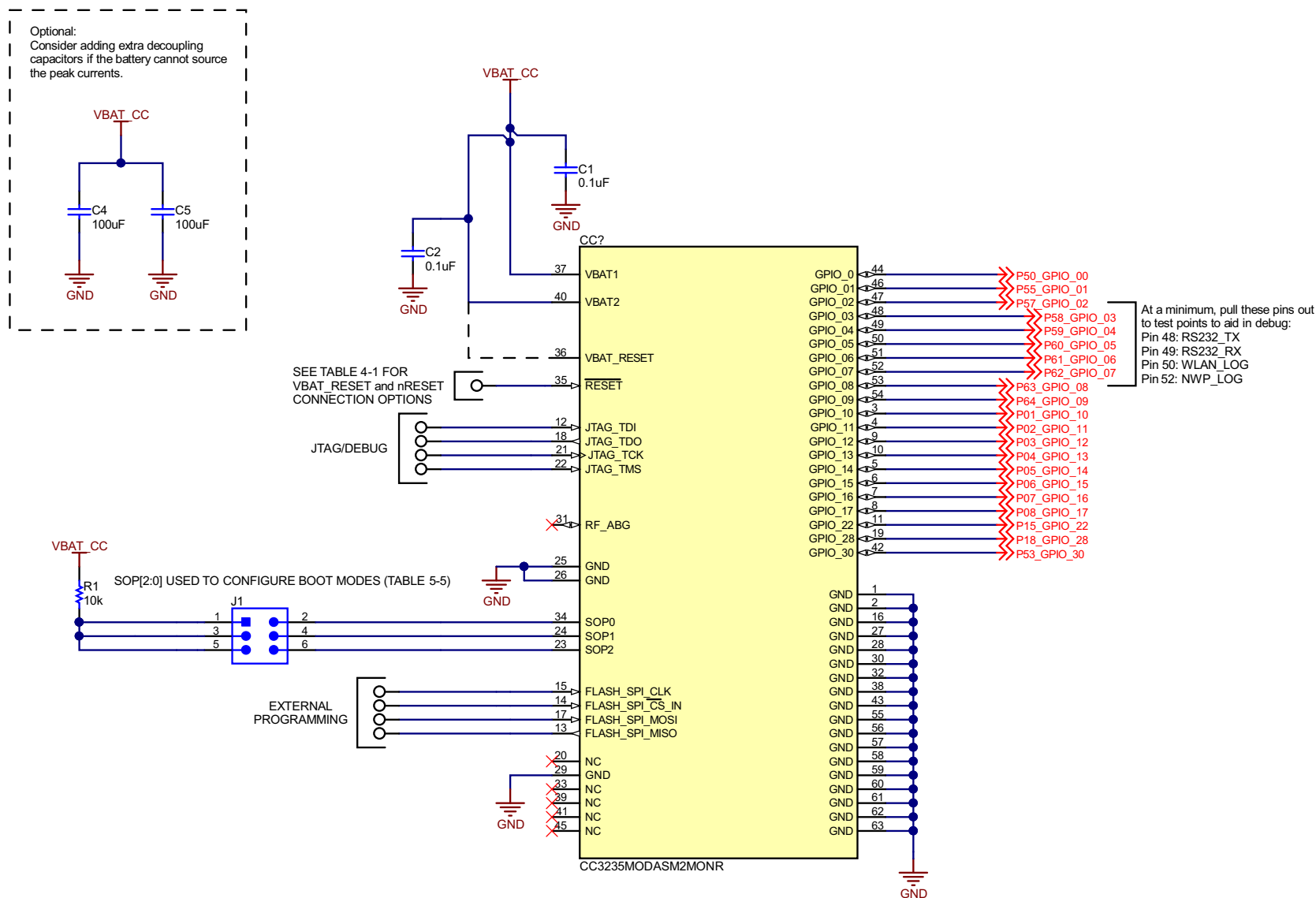
图 10-4. CC3235MODx Typical Application Schematic
