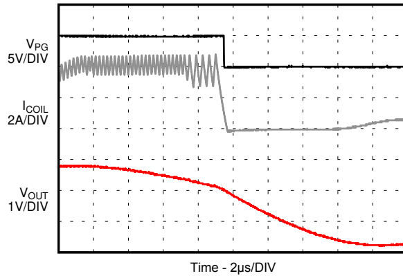
图 9-34. HICCUP Short Circuit Protection
