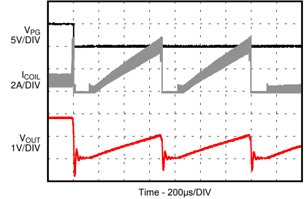
图 9-34. HICCUP Short Circuit Protection
