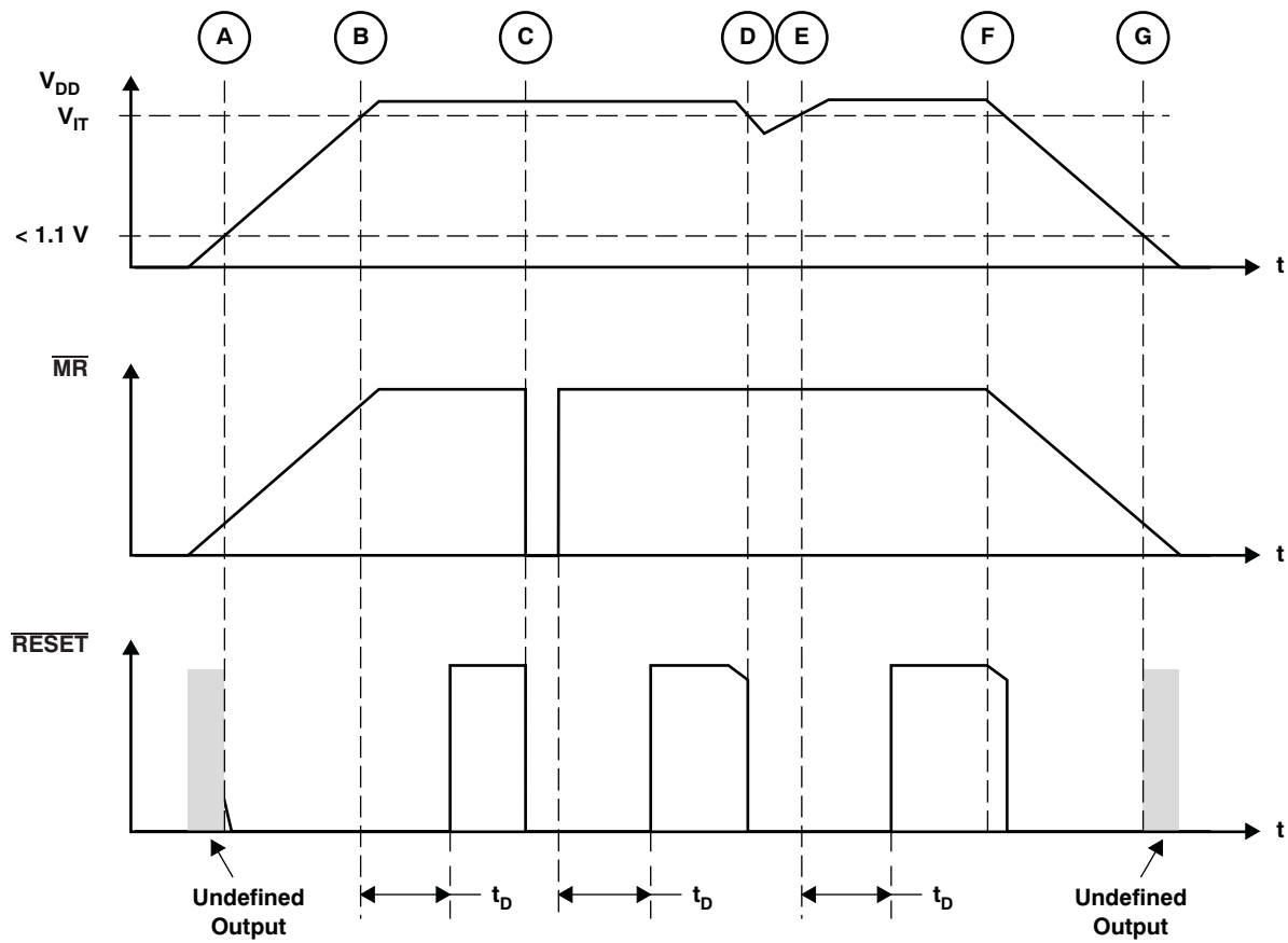
Figure 7. Timing Diagram
