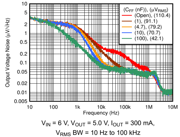
图 6-74. Output Noise vs Frequency and C_{\text{FF}}
