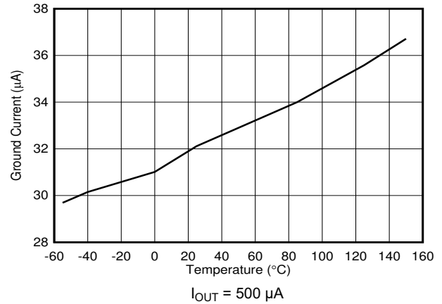
图 6-16. 500- \mu\text{A} Ground Current vs Temperature
