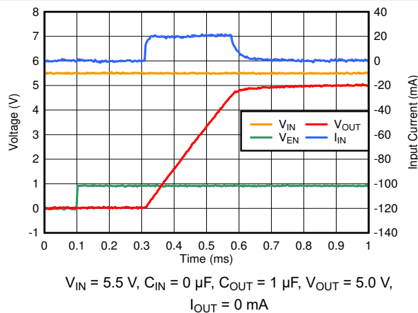
图 6-75. Start-Up Inrush Current With C_{\text{OUT}} = 1\text{ }\mu\text{F}
