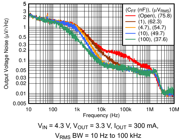
图 6-73. Output Noise vs Frequency and C_{\text{FF}}
