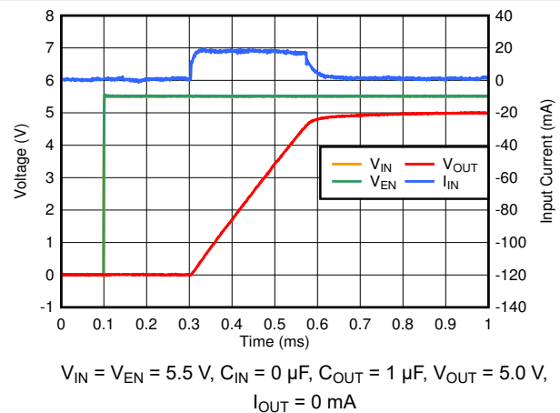
图 6-76. Start-Up Inrush Current With C_{\text{OUT}} = 1\text{ }\mu\text{F}
