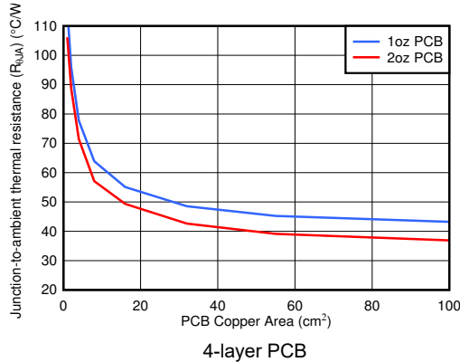
图 10-1. Junction-to-Ambient Thermal Resistance ( R_{\theta JA} ) vs PCB Copper Area
