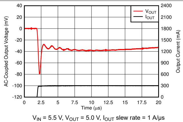
图 6-42. I_{OUT} Transient From 1 mA to 300 mA
