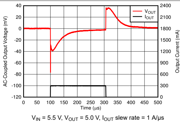
图 6-41. I_{OUT} Transient From 1 mA to 300 mA
