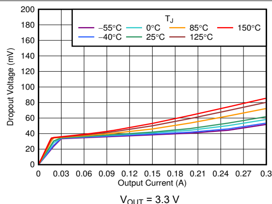
图 6-12. Dropout Voltage vs I_{\text{OUT}}
